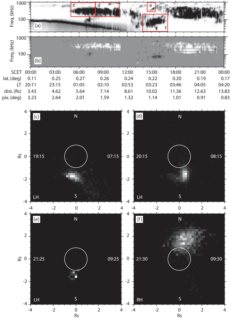
Figure 4: Direction Finding results for day 2005-089. (a) Flux dynamic spectrum summarizing all the radio emissions observed during the day in the 20–1000 kHz band. (b) Polarization measured for the same time frequency selection (white is LH, black is RH). Spacecraft time (SCET), latitude (lat.), local time (LT), distance to Saturn (dist.) and angular size of one map pixel (pix.) are shown under plot (b). The four lower plots are intensity maps with the selections: (c) 05:00–08:00 SCET, f > 150 kHz, V > 0.3 , \text{SNR} > 33 dB; \alpha_{xw} > 20^\circ ; (d) 08:00–11:00 SCET, f > 150 kHz, V > 0.3 , \text{SNR} > 33 dB; \alpha_{xw} > 20^\circ ; (e) 14:30–15:30 SCET, f > 150 kHz, V > 0.3 , \text{SNR} > 33 dB; \alpha_{xw} > 20^\circ ; and (f) 14:00–17:00 SCET, f < 150 kHz, V < -0.3 , \text{SNR} > 33 dB; \alpha_{xw} > 20^\circ . The white circles represent the size of Saturn, each pixel is 0.2R_S \times 0.2R_S at Saturn. The maps units are shown in R_S . The northern and southern direction as well as the mean local time at the limbs are shown at the border of each map.
