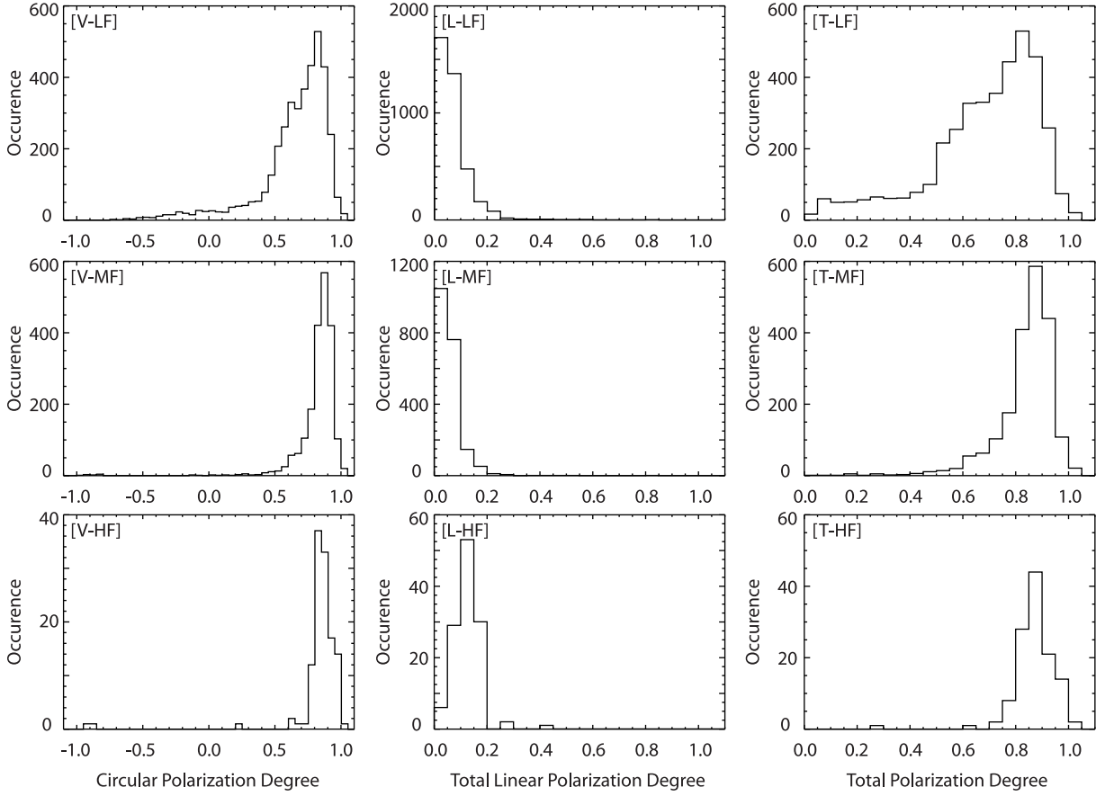
Figure 2: Polarization degree (V for circular, L for linear and T for total polarization degree) histograms for the three frequency band: LF (10–100 kHz), MF (100–325 kHz) and HF (325–1200 kHz). We have used data recorded between days 2004/002 and 2004/016 and computed the polarization degree through the polarimeter inversion, assuming the source position to be at Saturn. The SKR data has been selected with the following criteria: \text{SNR} > 20 dB on each antenna; \alpha_{xw} > 20^\circ . A total of 3865, 2051 and 121 samples is selected in bands LF, MF and HF respectively. The selected data represent respectively 0.3%, 0.02% and 0.005% of the total data sample for bands LF, MF and HF. Note that a 0.10 linear polarization degree bias appears in HF. It is an artifact due to both interferences lines and the small number of selected data.
